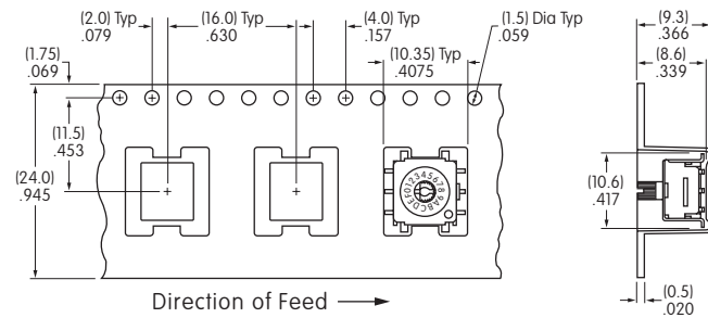
Tape Dimensions
